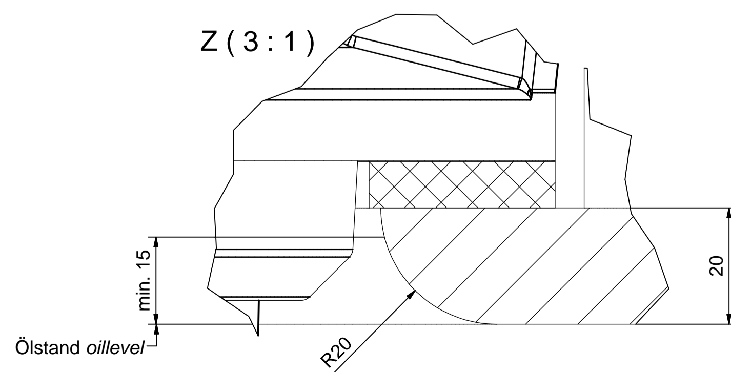
Alternativer Flansch alternative flange
