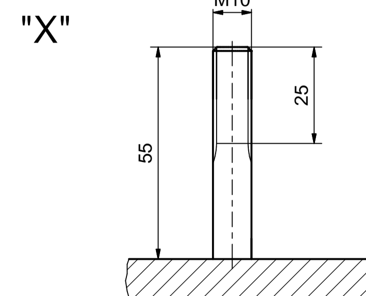
Befestigung nach DIN 42538 Flansch A Fastening in accordance with DIN 42538 flange A
