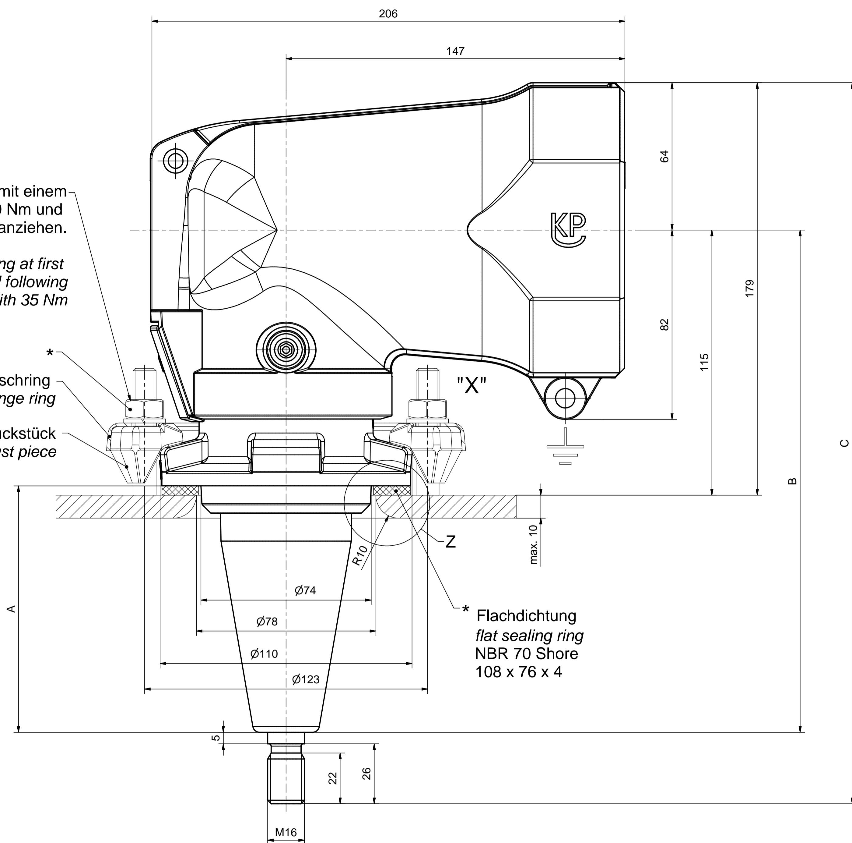
Befestigung nach DIN 42538 Flansch A Fastening in accordance with DIN 42538 flange A
