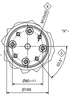
Ansicht / View "X"
